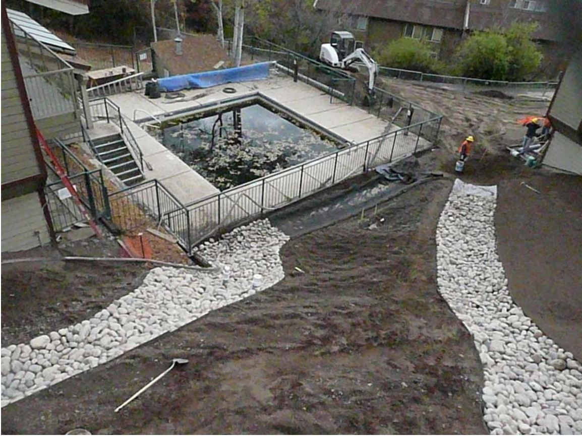
Rip rap Rock Drainage landscape Building A & pool
